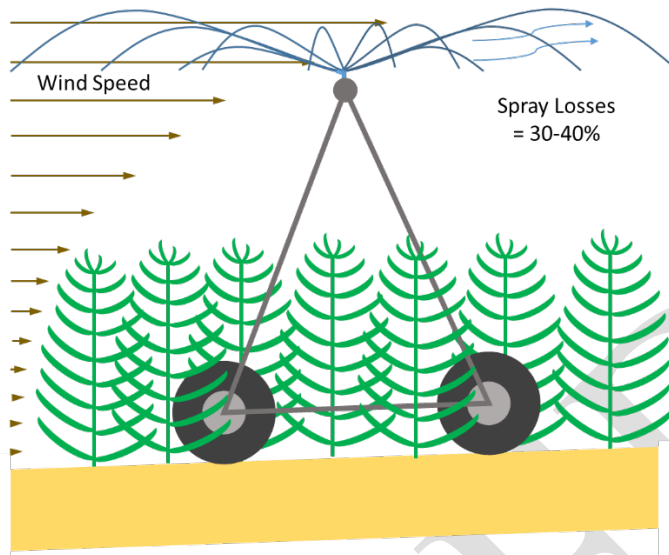
Figure 46. The water losses from sprinklers from traveling big guns, end guns, and impact sprinklers (especially those on top of a pivot) are typically from 30 to 40%. This is due to the higher wind speeds and greater wind mixing at higher heights, the higher sprinkler pressures dispersing the water, and because of longer water travel times through the air.
