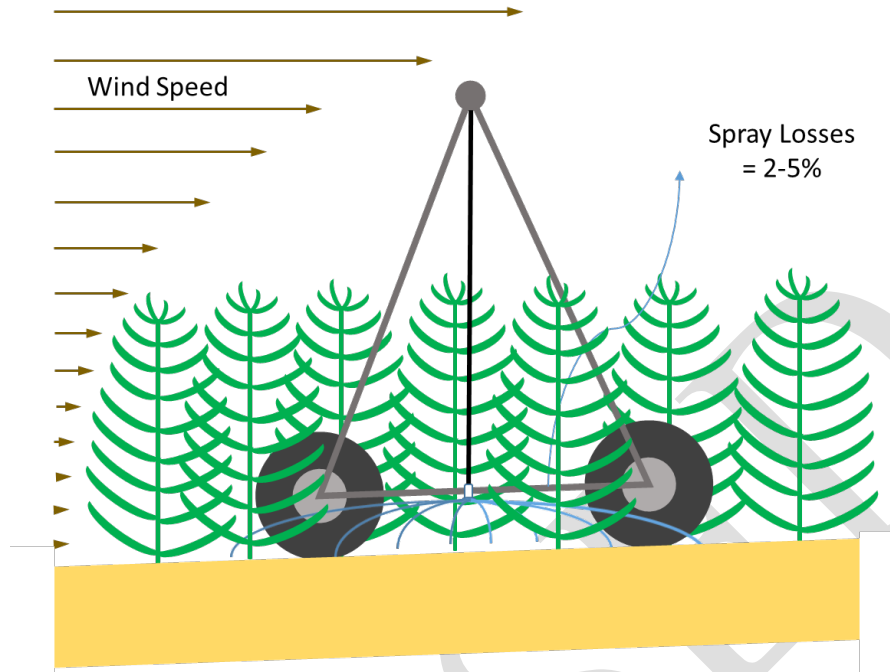
Figure 48. Low elevation spray application (LESA) or low energy precision application (LEPA) sprinklers emit water at low pressures near the soil surface and result in very little spray losses to wind drift and evaporation due to the low wind speed, low atmospheric mixing, higher humidity, low emission pressures, and very small time in the air resulting in very little mixing.
